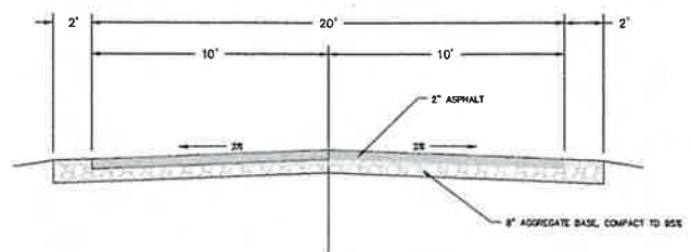
TYP DRIVEWAY SECTION NOT TO SCALE
